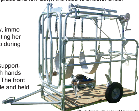
NB Pictured with optional Removable Handles and Braked Winch.
